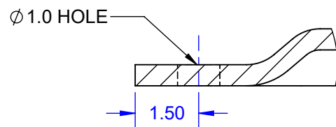
DETAIL E SCALE 8 : 1
